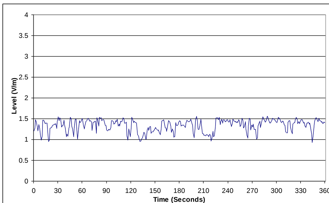
Electric field strengths recorded over 6 min period using 18 GHz probe at point of max NIR:
